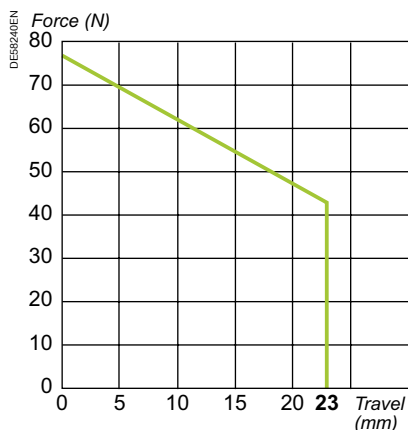
Value of the force provided by the striker according to its length of travel.
